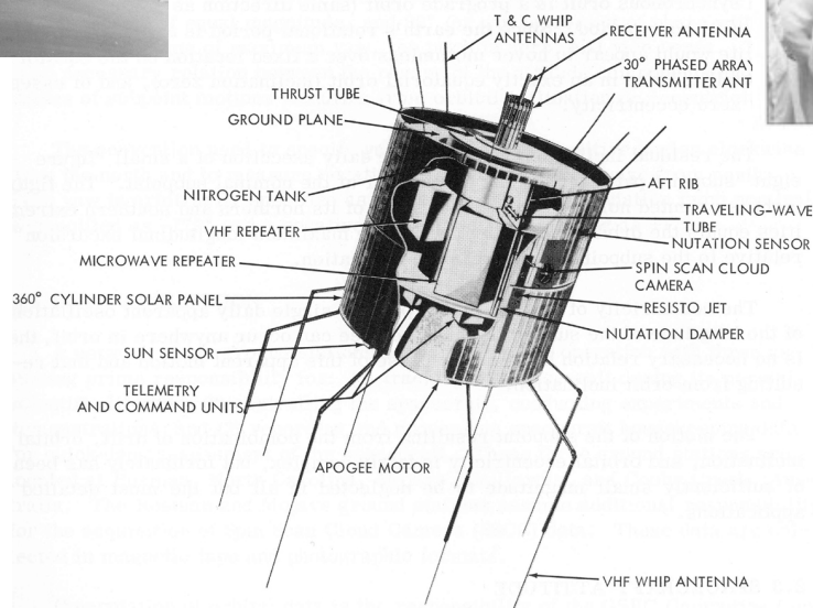
Figure 2-1. Applications Technology Satellite (ATS-1).
